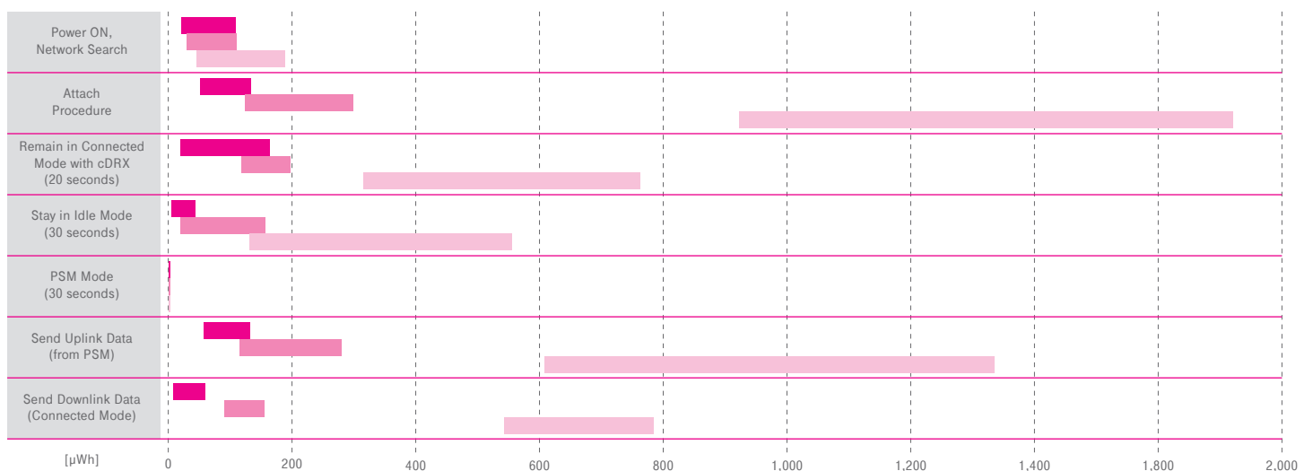
Figure 3: Power consumption of common radio chipset routines
